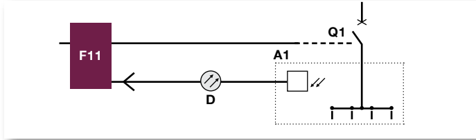
F11 Arc Monitor, Q1 Circuit breaker, A1 Switchgear, D Detector
